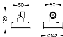
Round base for Ground mount (1-10V or Dali) [pre-assembled from factory] Ordering Code/รหัสสั่งซื้อ : AUN-MOT-0022-XX
