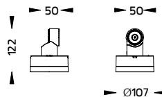
Round base for Ground mount (On,Off) [pre-assembled from factory] Ordering Code/รหัสสั่งซื้อ : AUN-MOT-0021-XX
