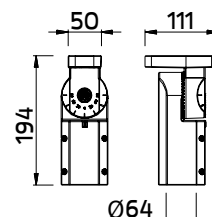
Adaptor installation
