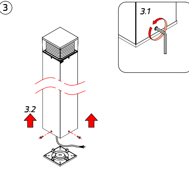
TOWER3 - Bollard
