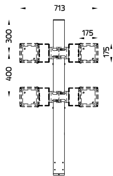
Pole Array for 4 Spotlights. Ordering Code : 0507-0-9-000-XX
