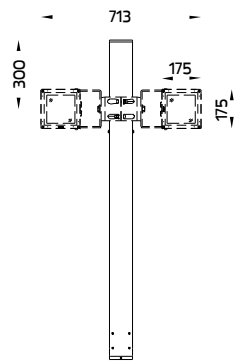
Pole Array for 2 Spotlights. Ordering Code : 0506-0-9-000-XX
