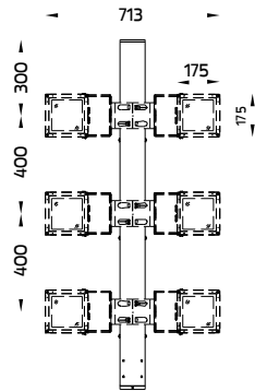
Pole Array for 6 Spotlights. Ordering Code : 0508-0-9-000-XX
